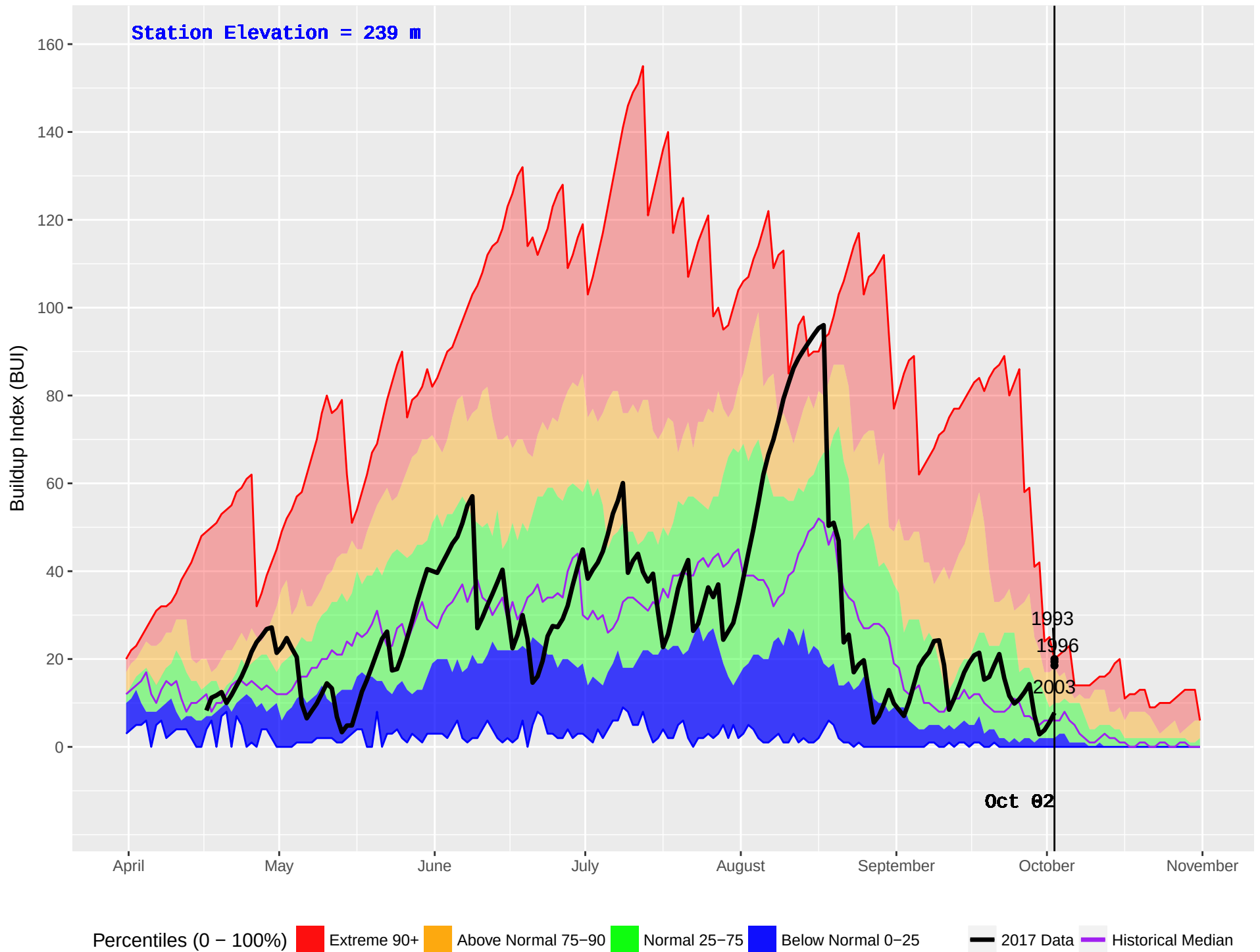
ROSSWOOD (105) : Historical (1970–2016) and Current (2017) Noon Buildup Index (BUI)
