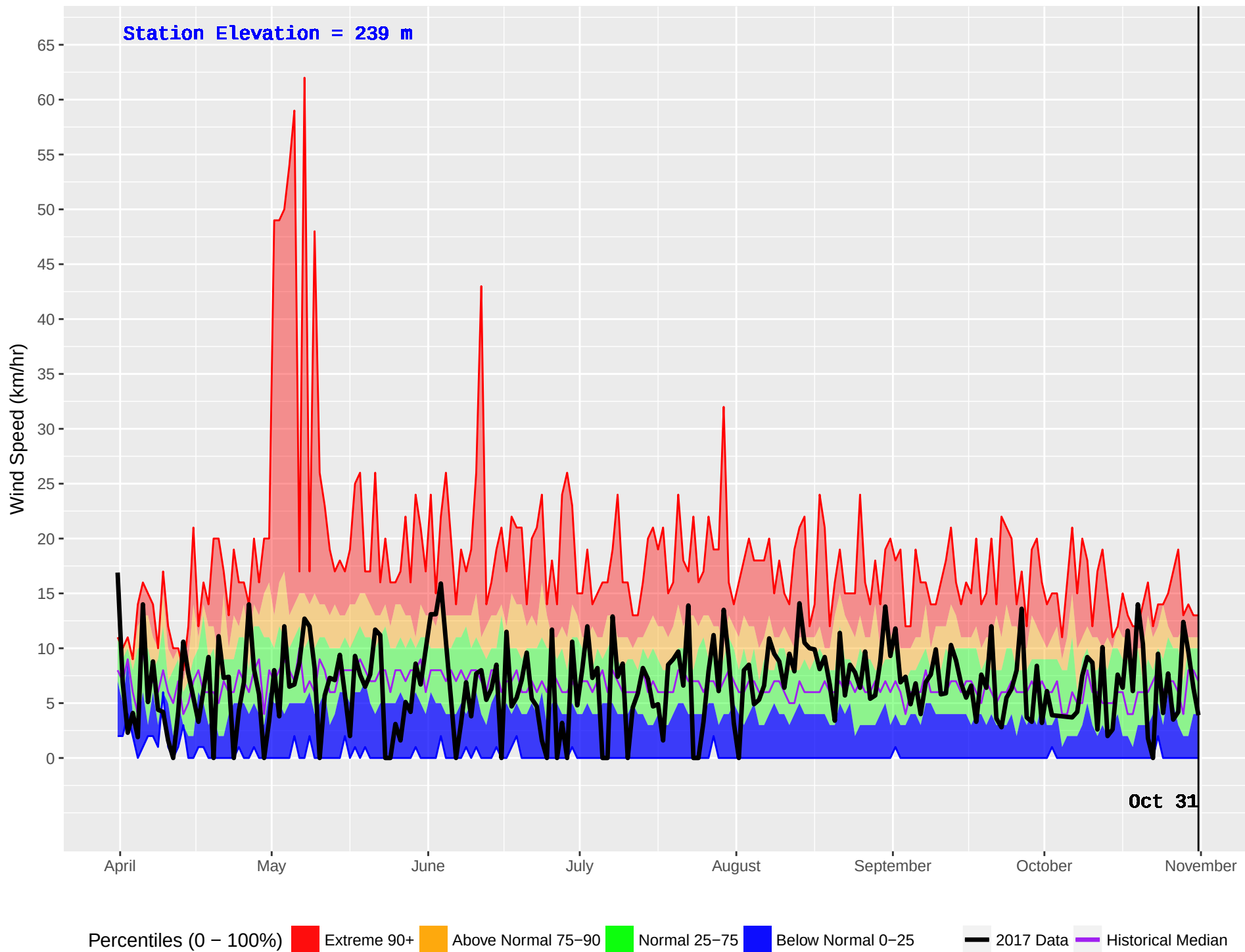
ROSSWOOD (105) : Historical (1970–2016) and Current (2017) Noon Wind Speed
