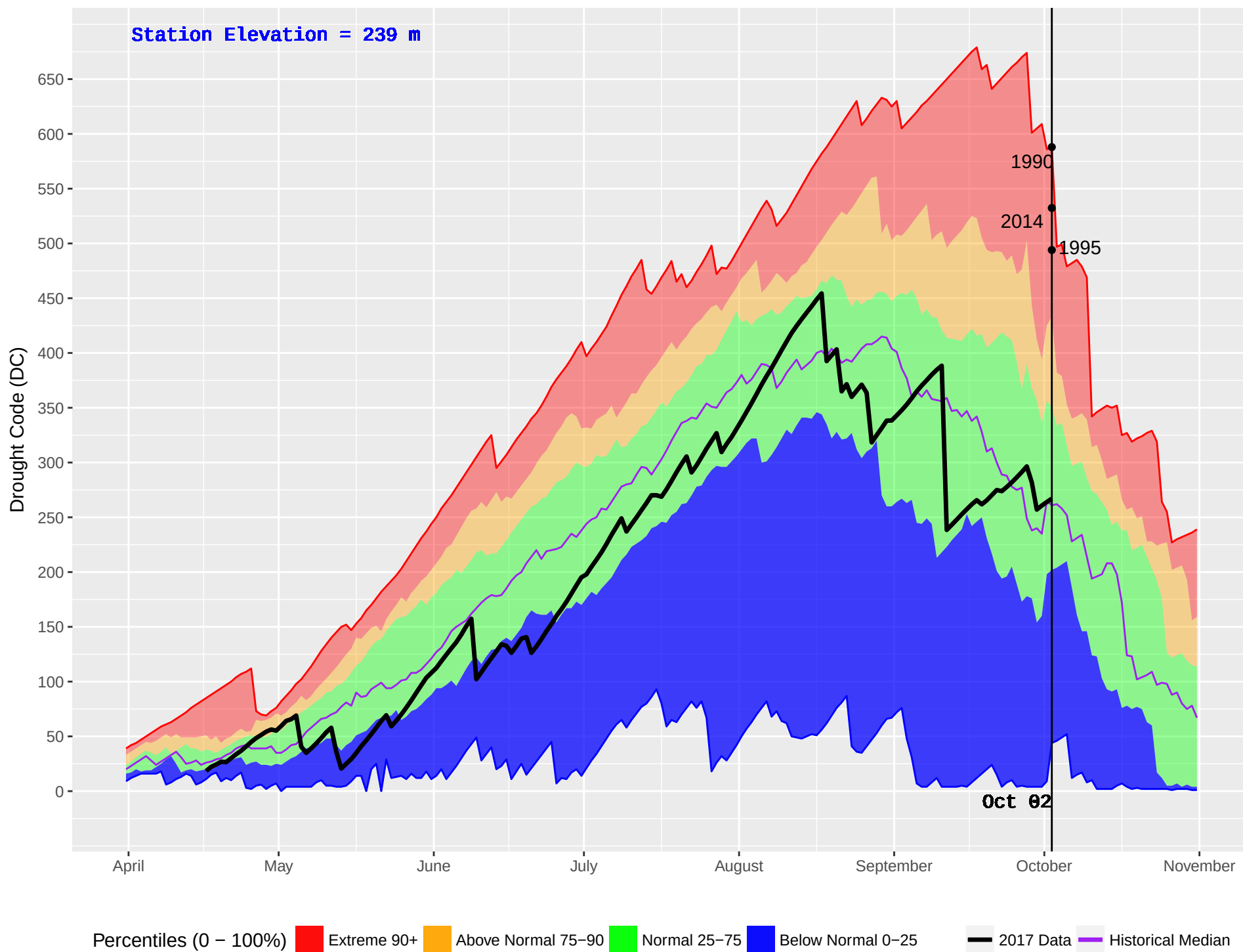
ROSSWOOD (105) : Historical (1970–2016) and Current (2017) Noon Drought Code (DC)
